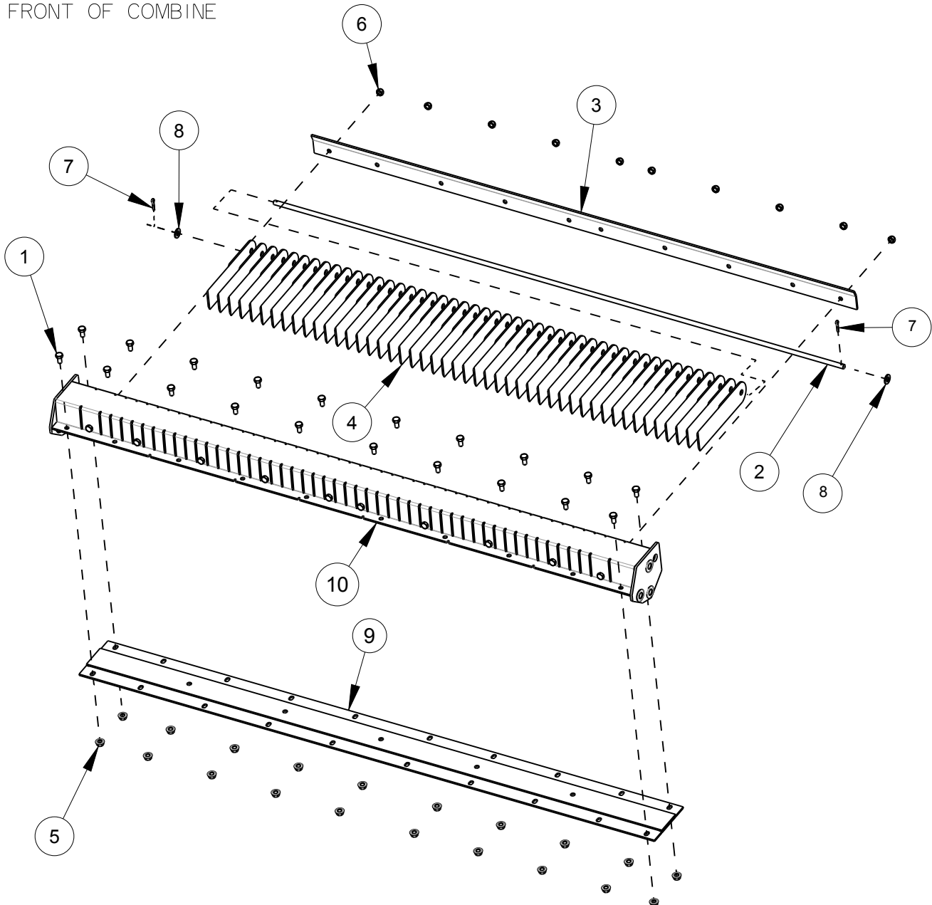
CG352CA - Knifebar Assy MAV 55L W/O Paddles - Charcoal
