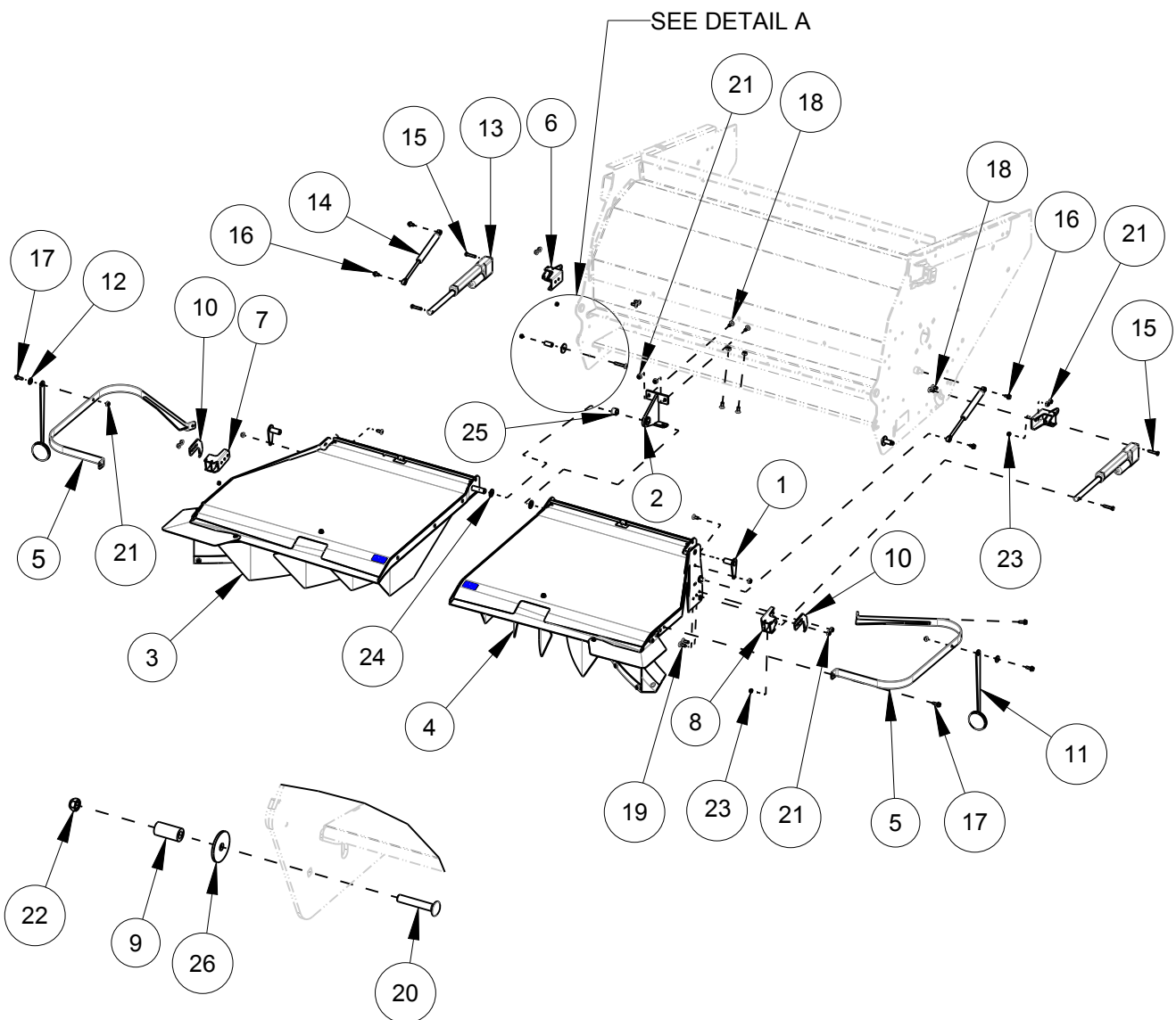
DETAIL A
