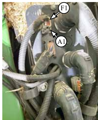
600 Series Adapter Harness (G)
