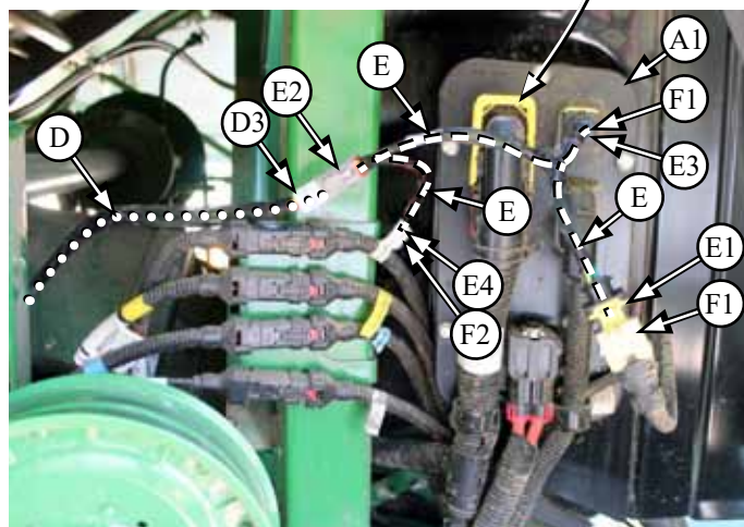
S700 Series Shown
