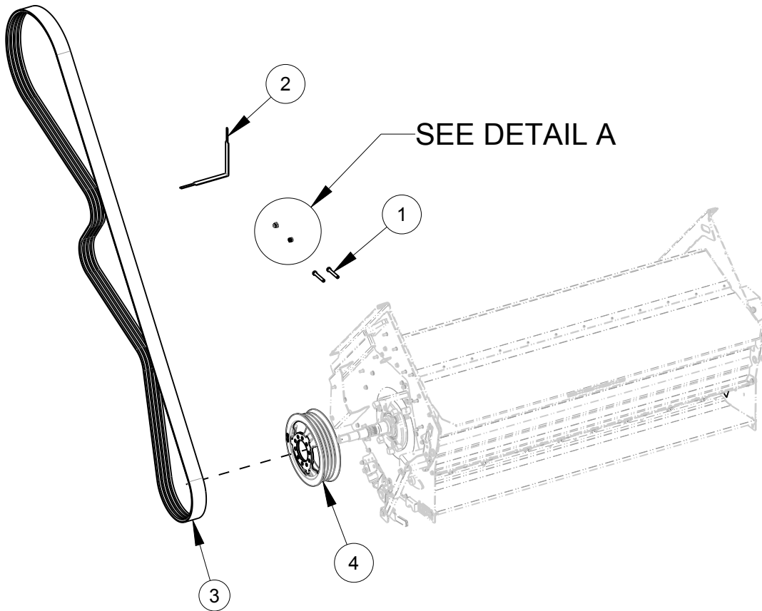
DETAIL A
